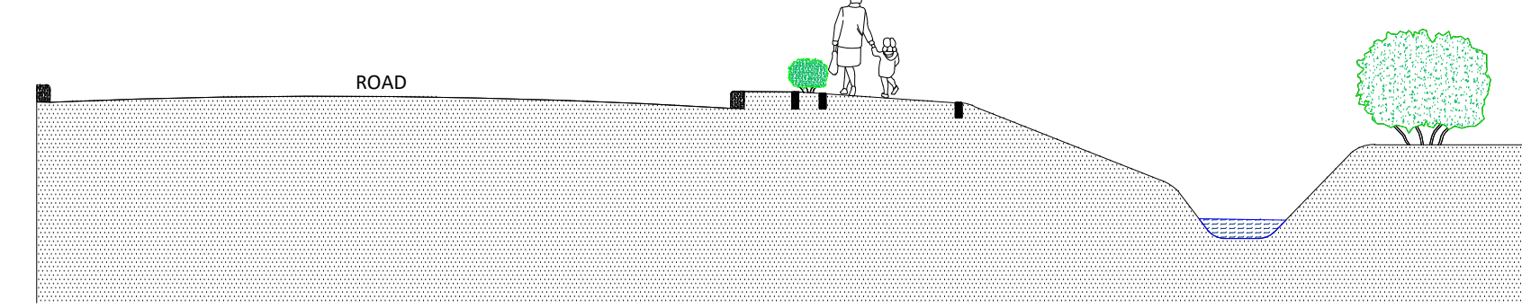
SECTION E-E
