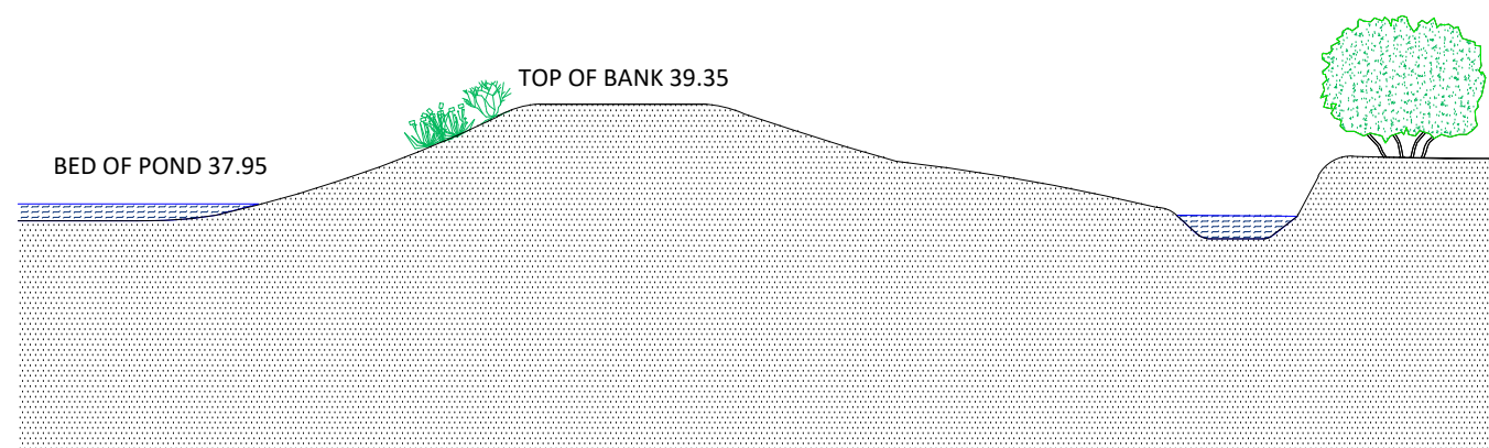
SECTION C-C
