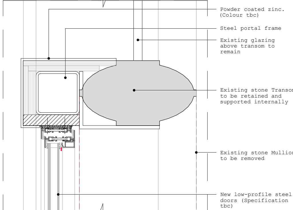
Detail 02 - 1:5
