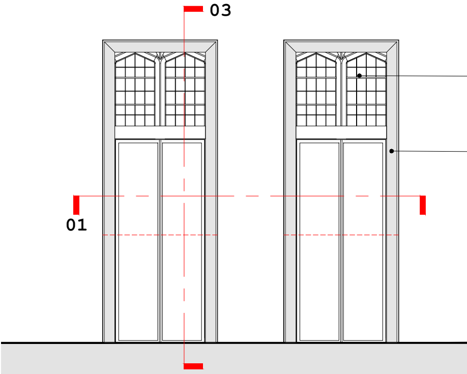
Internal Elevation - 1:50
