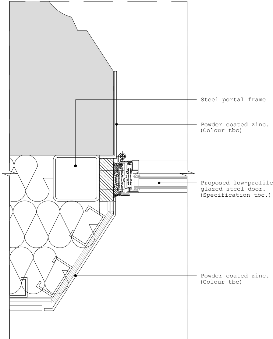
Detail 01 - 1:5
