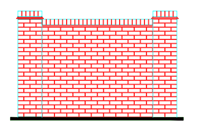
1.8m high Brick Screen Wall 1.8m high Closeboard Fence 0.6m high Knee Rail Fence 1.8m Green Fence
